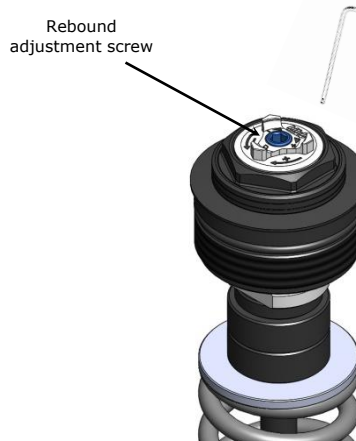
Right fork leg With Rebound adjustment
